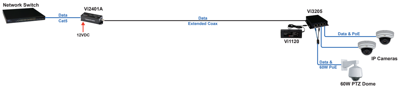
The Vi3205 can receive data over extended distance Coax up to 3,000 ft. at 100Mbps and power 60W PoE cameras using the Vi0015 combiner cable and a local power supply.
