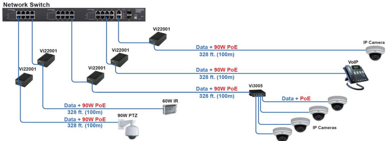
The Vi22001 can be used to power a wide variety of high PoE power devices with Single or Dual PDs.
