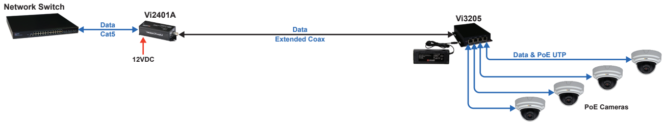
The Vi3205 can receive data over extended distance Coax up to 3,000 ft. at 100Mbps and power 4 PoE cameras using local power supplies.
