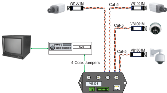
Vi6204: 4-Channel AVC Active Receiver
