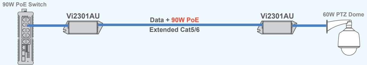
The Vi2301AU extends Ethernet and 90W PoE from a PoE switch.
