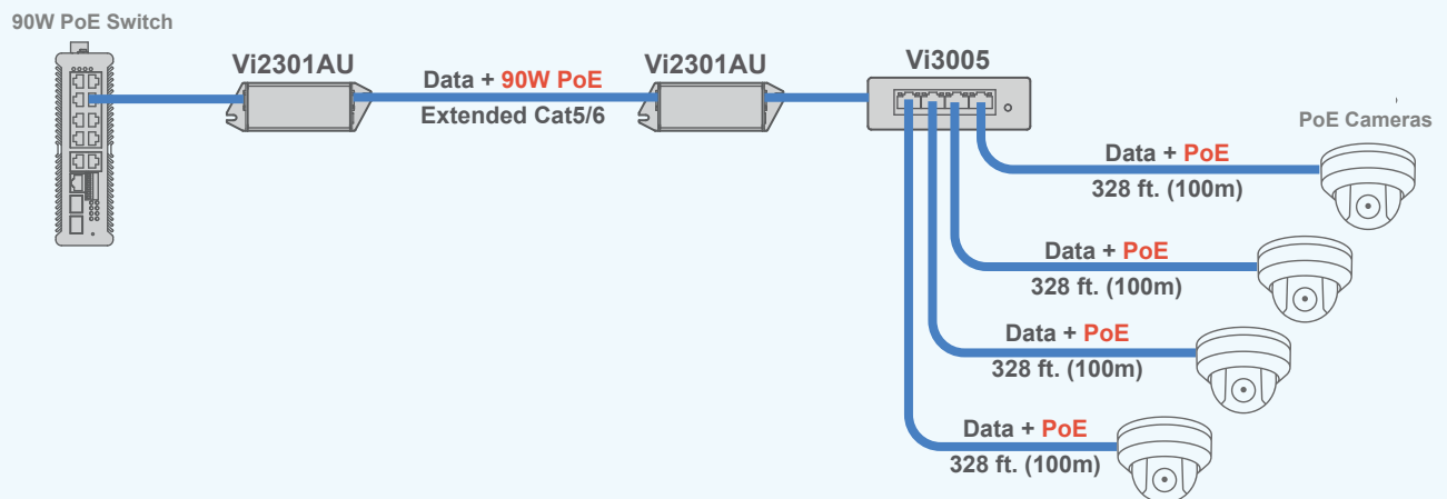
The Vi30002U can be used to connect multiple PoE cameras at extended distances.
