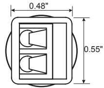
Left View
