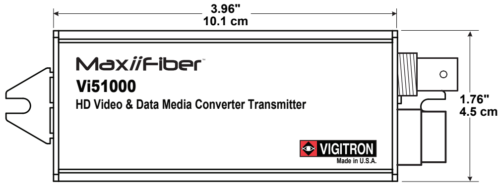
Top View
